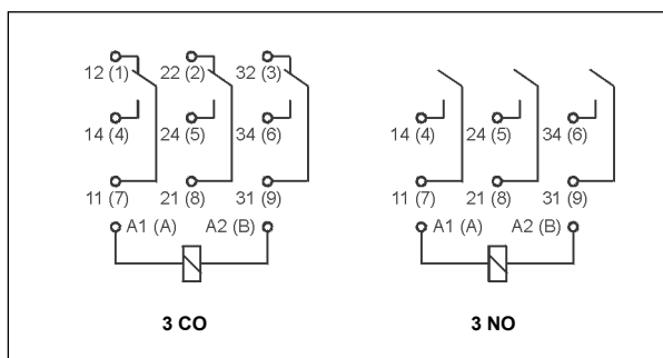
Connection diagrams (pin side view)
