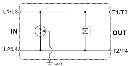
Connection diagram
